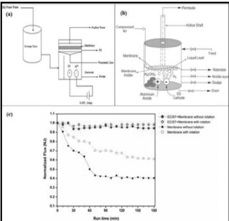
Fig. 2: (a) Schematic process flow diagram for the operation of ECEFMM; (b) Schematic diagram for the working principle of ECEFMM; (c): Comparative analysis of variation of normalized permeate flux (NJ) with time at different modes of operation.
