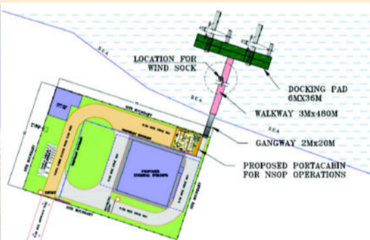
Site Layout for Shaheed Dweep for NSOP
